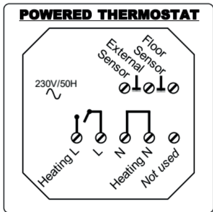
Internal Wiring Diagram
